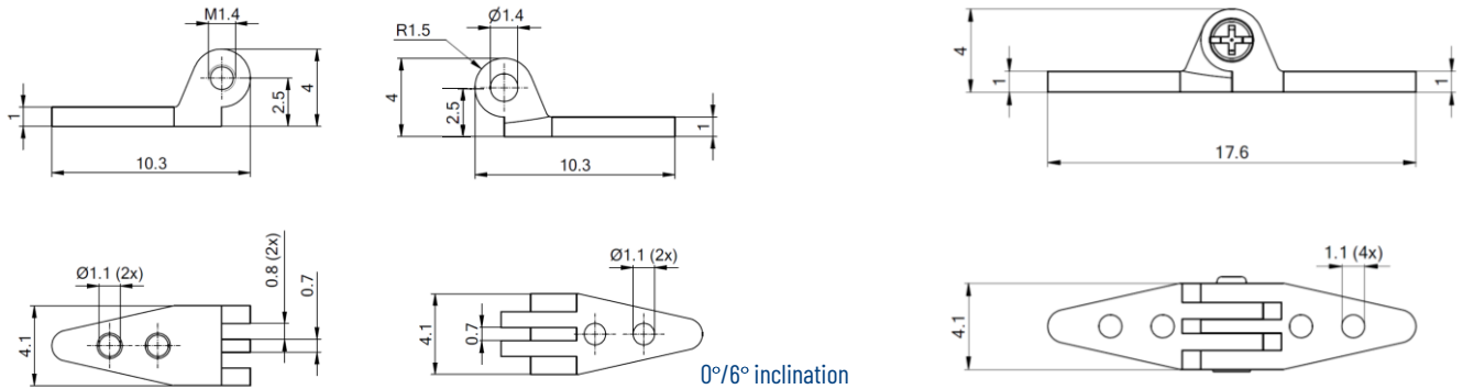
Diamond Rivet hinge 51-05126.90X.01/02/03
