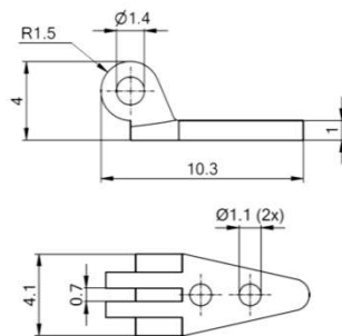
Diamond Rivet hinge 51-05126.90X.01/02/03
